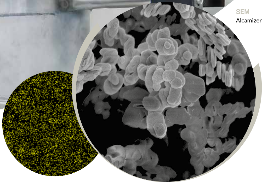
SEM/EDS - ALUMINIUM SCAN Excellent dispersibility of Alcamizer in the PVC matrix
